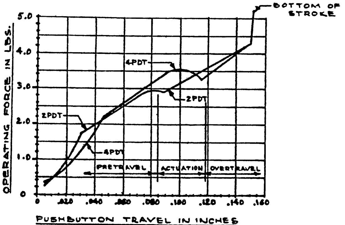
Typical operating force v/s plunger travel (for Ref. only)
