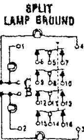
Schematic Diagram Models 49, 59, and 89 (09, 10, and 11)
