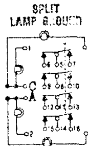
Schematic Diagram Models 49, 59, and 89 (12, 13, and 14)
