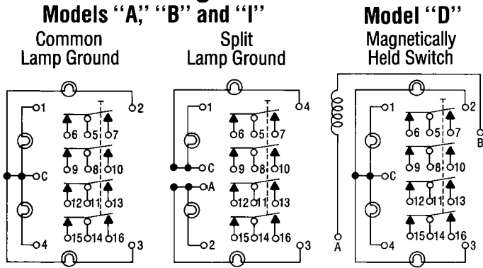
Pushbutton switch schematic 4PDT Shown. For 2PDT, Omit terminals 8-13. For Indicator, Omit terminals 5-16.
