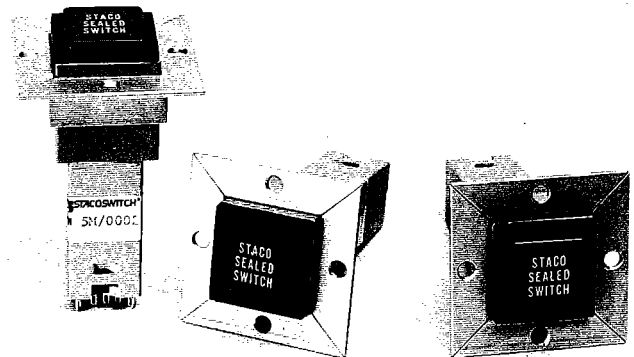
Single station, rear mount housing, Series 505M Crimp Pin Terminal Matrix, right and center; and a Series 5M Matrix with solder termination receptacle, left. Units have dripproof pushbuttons installed.
