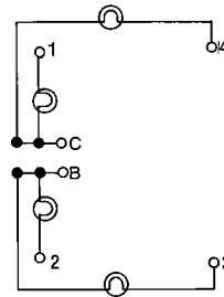
Split Lamp Ground
