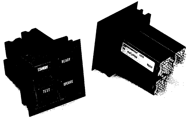
Series 5M Dress Bezel Housing with modules and pushbuttons installed. Unit shown has three "D" solenoid-held switches and one "A" switch. See note at bottom of page 9 Ordering Information when specifying system with "D" and "A", "B", or "I" modules and/or common and split lamp grounds.
