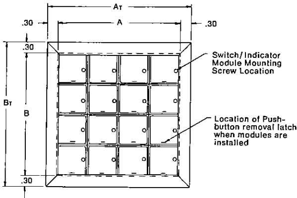
RECOMMENDED PANEL MOUNTING DETAIL
