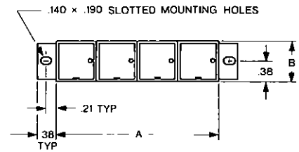
VERTICAL FLANGES
