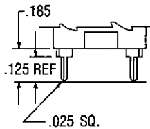
Style P Printed Circuit Terminal
