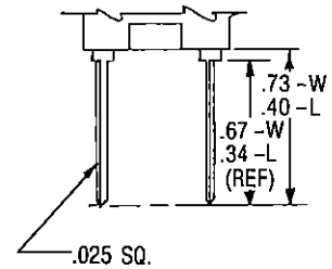
Style W/L Wire Wrap Terminal
