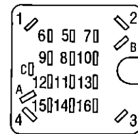
Terminal Arrangement
