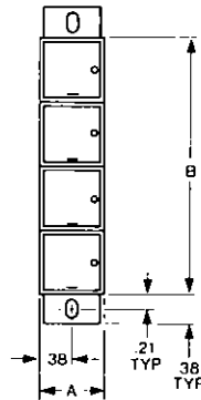
HORIZONTAL FLANGES
