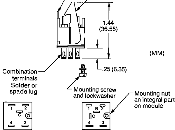
Terminal Arrangement
