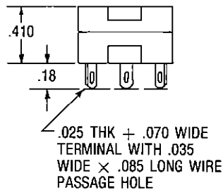
Style S Solder Terminal
