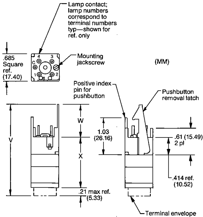
HEIGHT DIMENSIONS
